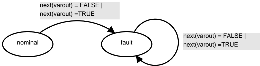
Figure 3.15: EM for a non-determinism by reference fault mode for boolean variables
